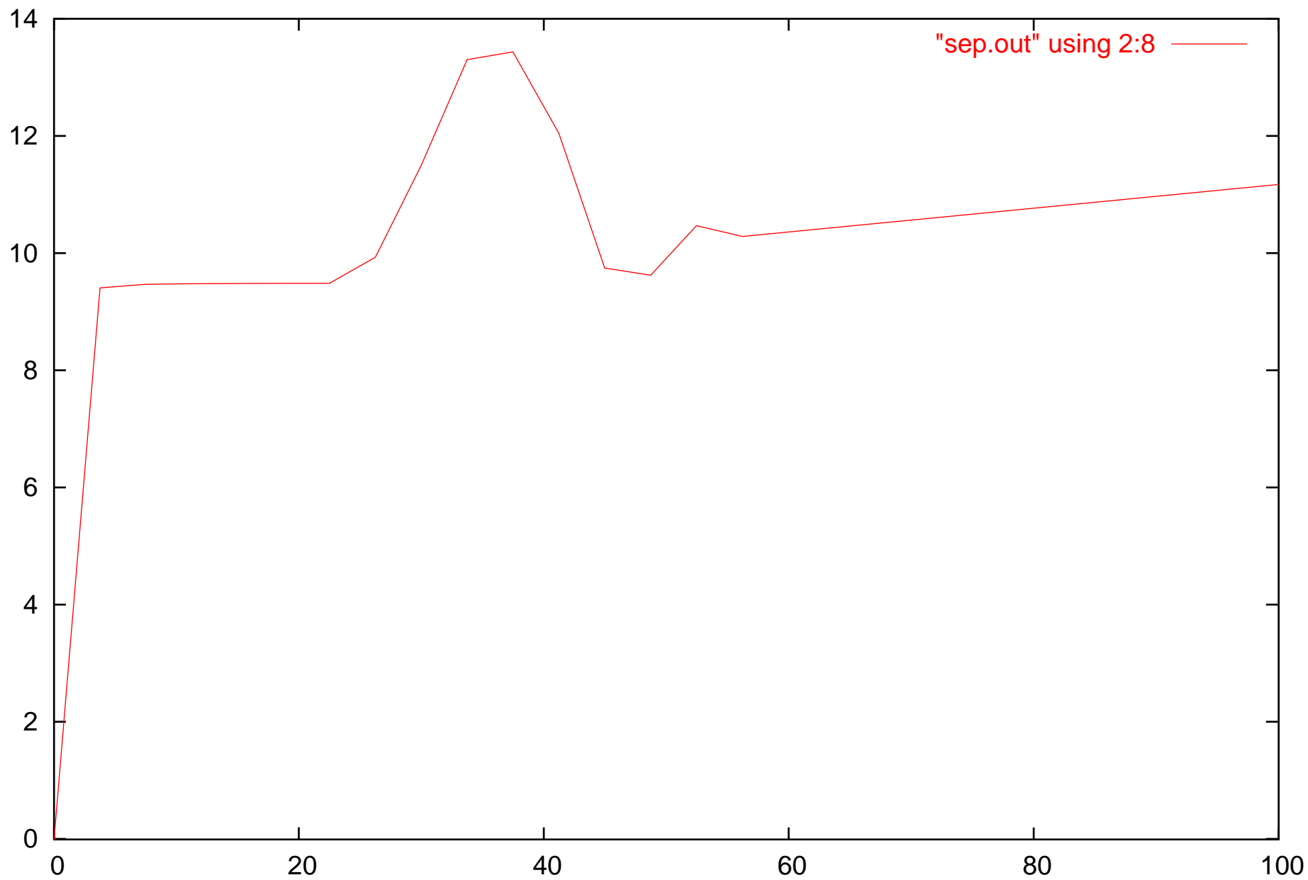
Separation long range IP1: normalized to minimum beam size
