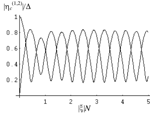
Figure 6. Envelopes of the total centroid displacements after a kick at one of the beams
