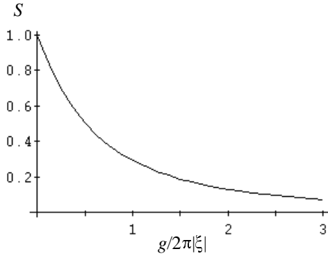
Figure 8. Continuum modes suppression factor due to feedback.
