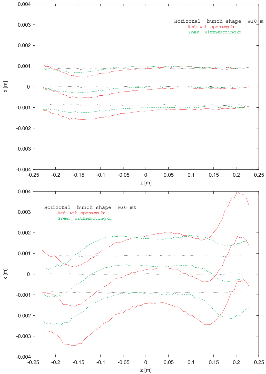
Figure 1: Simulated horizontal bunch shape (centroid and rms size) after 10ms (top) and 30ms (bottom).
