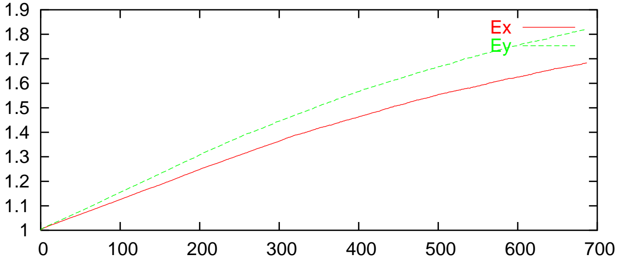
Emittance vs #turn
